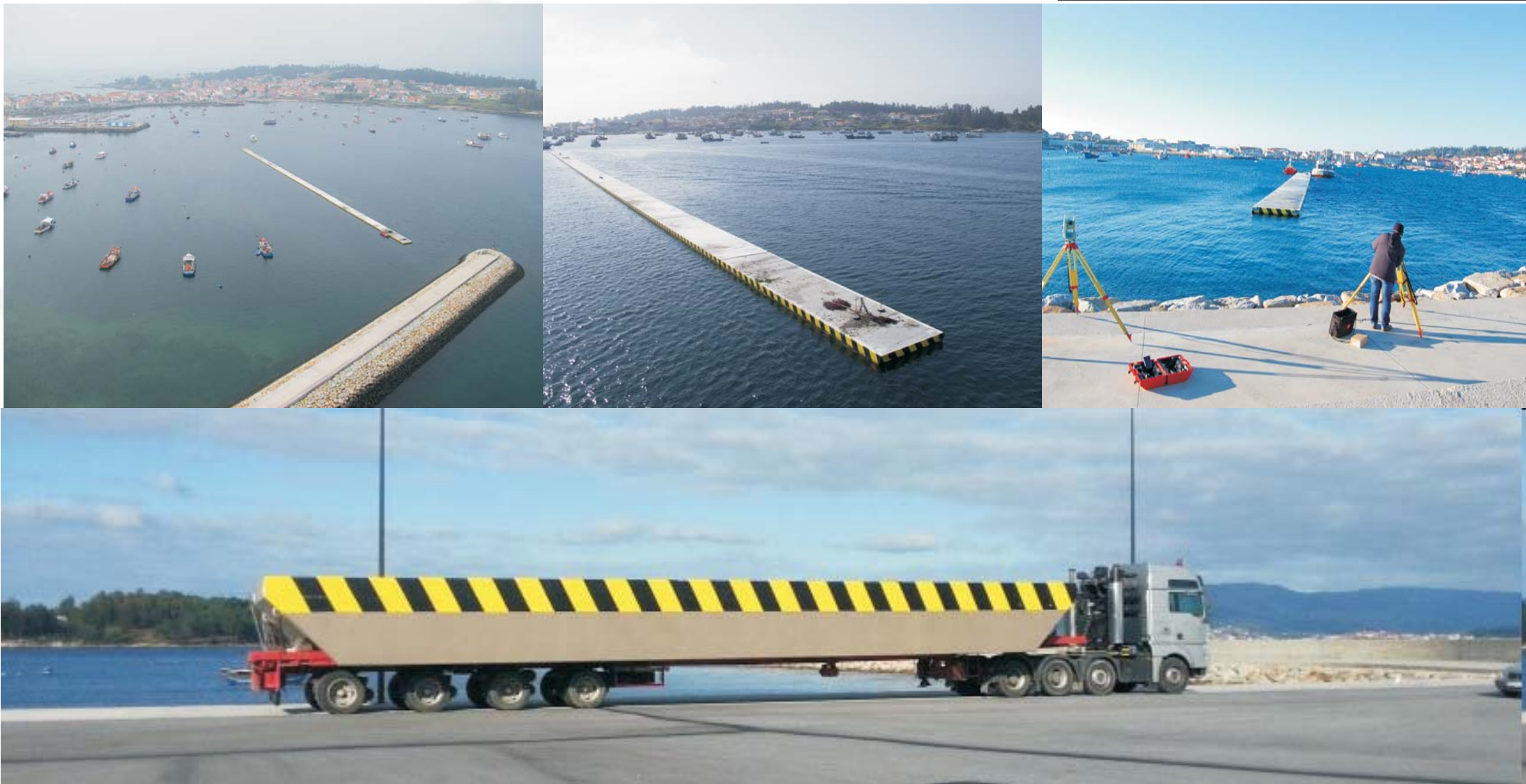
FLOATING BREAKWATER IN XUFRE'S PORT
